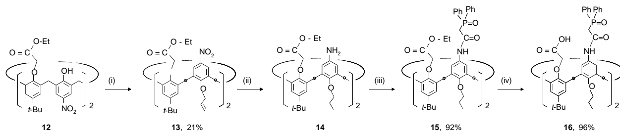
Scheme 2. Synthesis of 1,3-alternate derivatives combining two CMPO with two carboxylic groups. (i) Allylbromide, Cs 2 CO 3 , DMF, 50°C; (ii) H 2 , Raney-Ni, THF, r.t.; (iii) AE1 , CH 2 Cl 2 , r.t. and (iv) LiOH, THF–MeOH, r.t.
